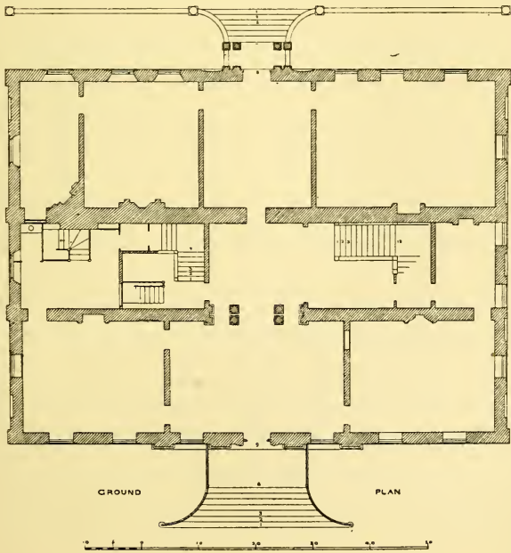
PLANS OF ELTHAM CLUB-HOUSE.
